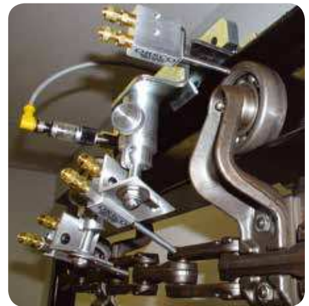
Image 1. Both the chain pins and wheel bearings on this overhead conveyor are being lubricated with four nozzles. A proximity switch times the intermittent spray to only lubricate the wear points.
